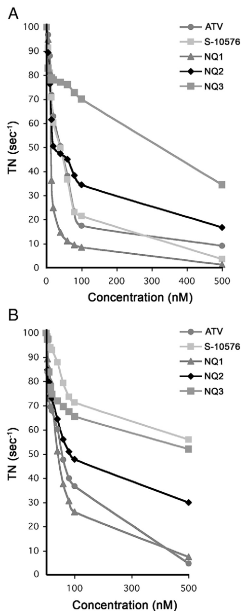
Fig. 3. Effect of 2-hydroxy-naphthoquinones on bc_1 activity of (A) yeast and (B) bovine bc_1 complexes. The cytochrome c reductase activity of purified enzyme was measured as described in Materials in the presence of increasing concentrations of inhibitor. The assays were performed in duplicate and the results are shown as averages. Activities are expressed as a percentage of the turnover number of each strain in the absence of inhibitor.
