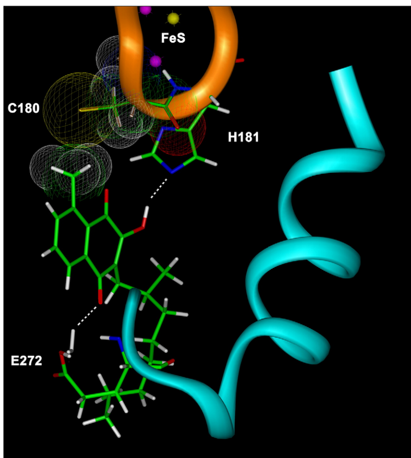
Fig. 2. Structure of 2-OH-3-(2-Me-octyl)-8-Me-naphthoquinone (NQ2) docked in the ubiquinol oxidation pocket at center P. Portions of the Rieske protein and cytochrome b are shown as gold and cyan ribbons, respectively. Van der Waals radii depicting the non-covalent interaction between the 8-methyl group of the naphthoquinone ring and Cys-180 (C180) of the Rieske protein are shown. The hydrogen bond between the 2-hydroxy group of NQ2 and His-181 of the Rieske protein and the water-mediated hydrogen bond between the 4-carbonyl oxygen of NQ2 and Glu-272 of cytochrome b are indicated by dashed white lines. Carbon atoms are shown in green, oxygens are red, hydrogens are white, nitrogens are blue, sulfurs are yellow, and iron is purple. The structure was created by substitution of NQ2 into the stigmatellin liganded crystal structure of the yeast bc 1 complex [23] and energy minimization as described in the Experimental procedures.
